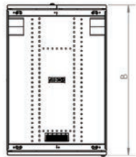
Top view (600mm width)
